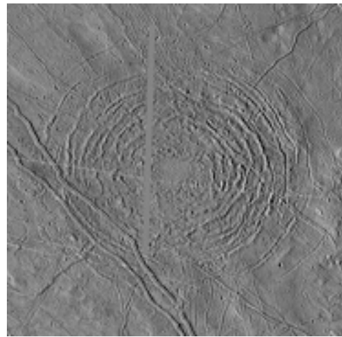
Tyre Crater
