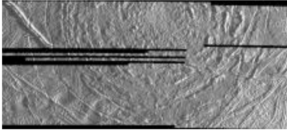
Callanish Crater
