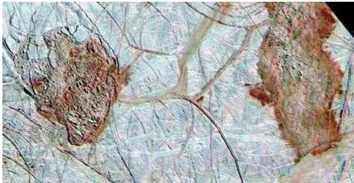
Thera & Thrace Macula
