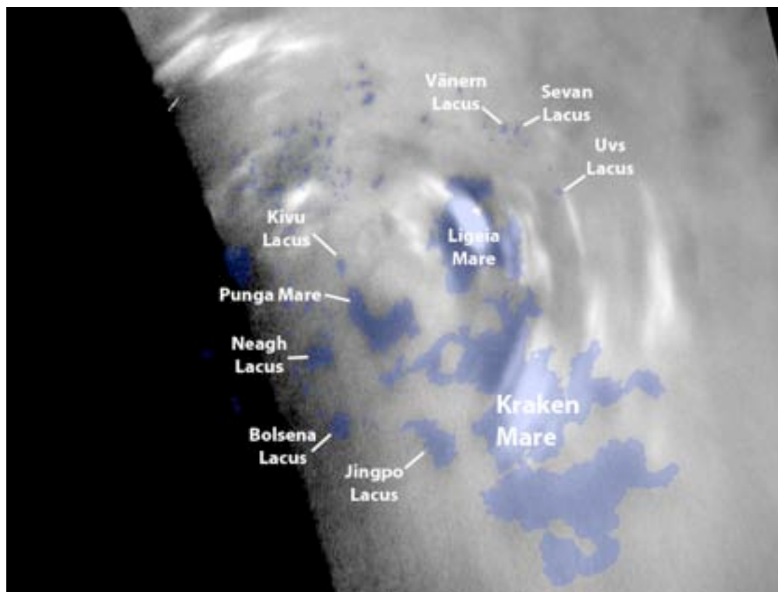
Lakes on the North Pole of Titan
