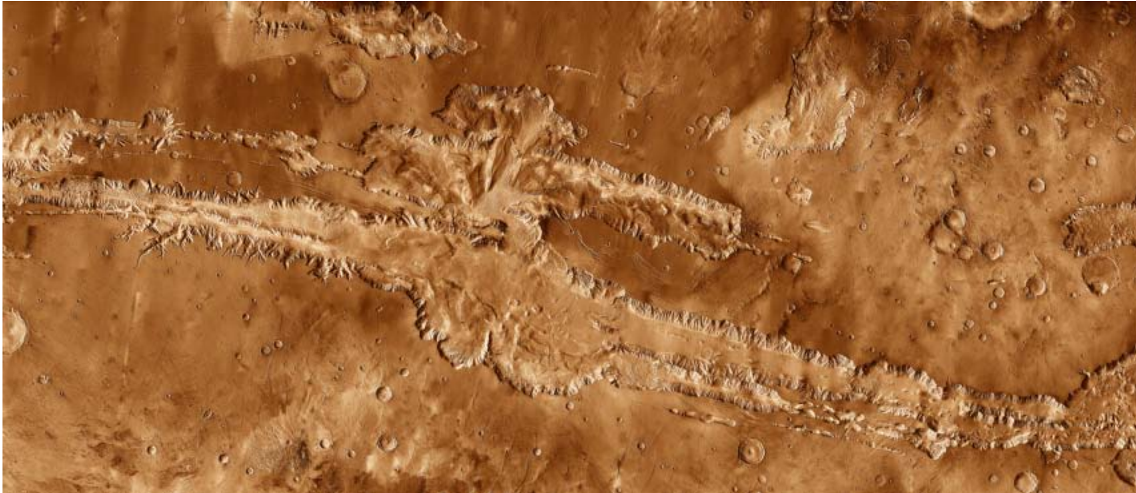
Valles Marineris, a large canyon on Mars.
