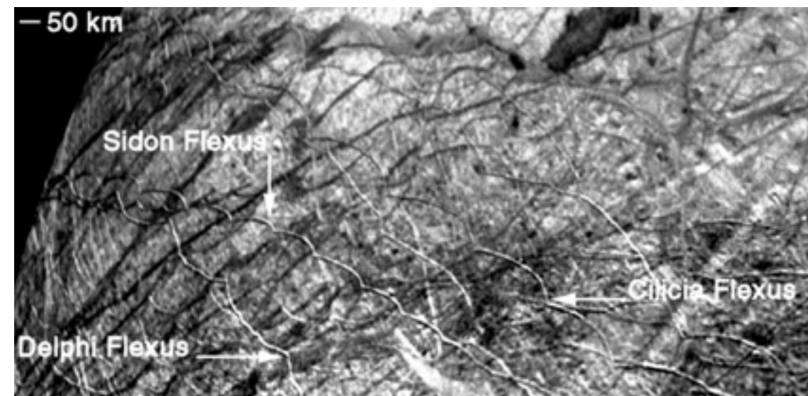
Cycloids
