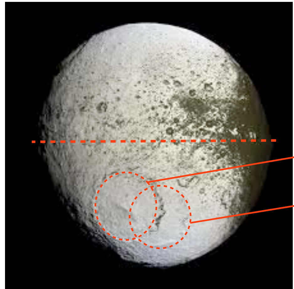
Saragossa Terra (Southern lighter hemisphere)
