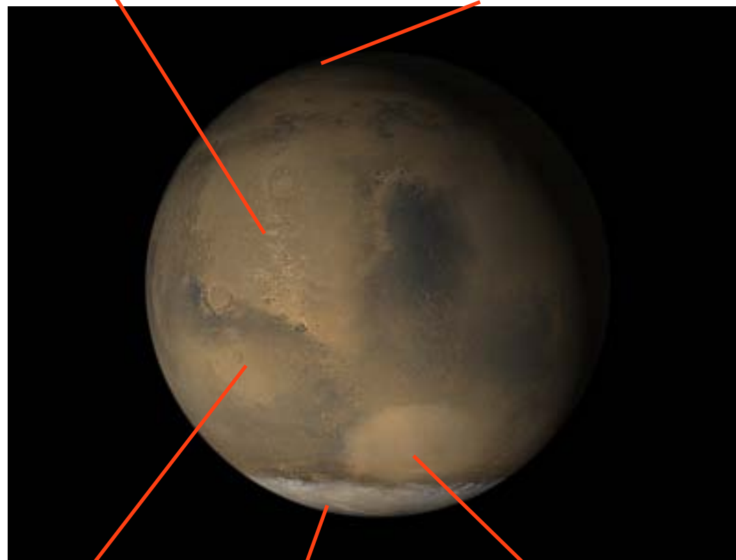
Margaritifer Terra
