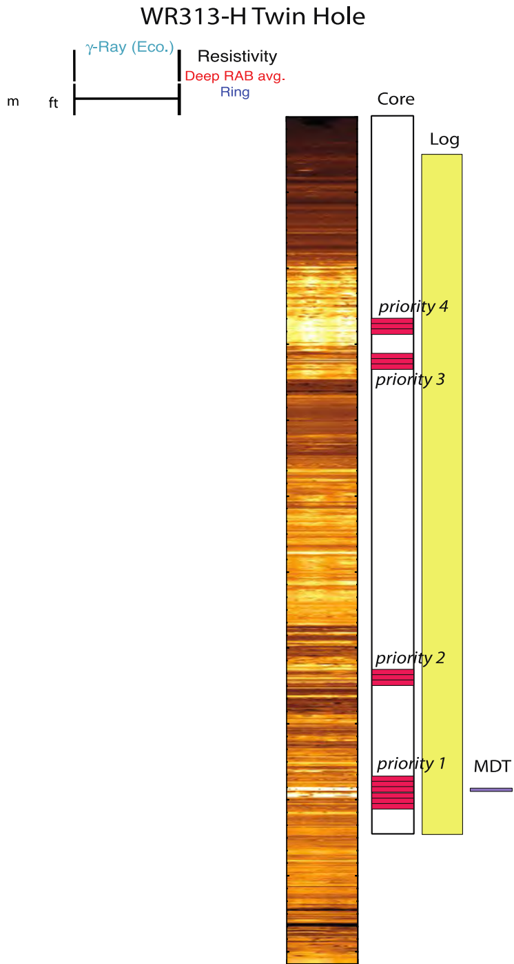
Figure 4: The WR 313-H hole was previously drilled. Our target locations are labeled Priority 1 and Priority 2 for this drilling project. See Table 1 and Table 3.
