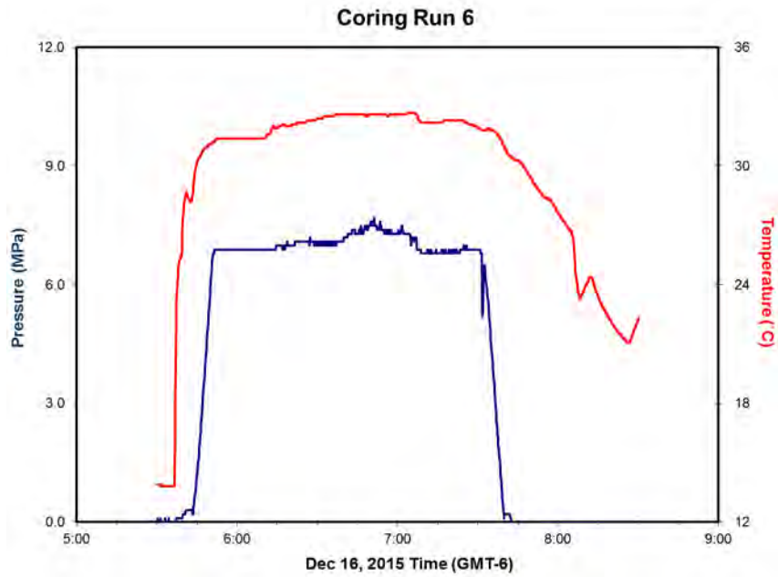
Figure B5: DST data from Coring Run 6.
