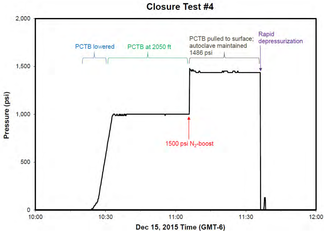
Fig 5: DST pressure from Closure Test 4.
